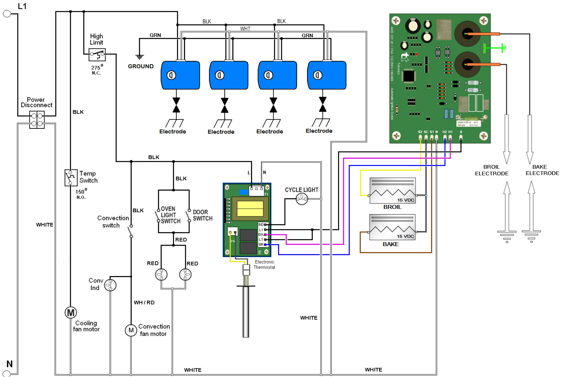
DCCG130-4B FREESTANDING GAS RANGE Schematic Diagram
